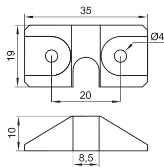
No. # 14.02.010 - 0,54 лв Plastic Drawer Stop for Central Locks Black cc 20 mm
